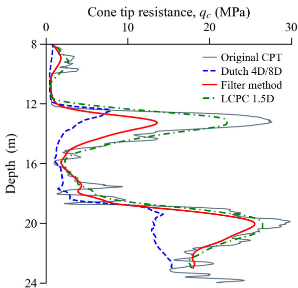
Fig. 6. Three different averaging methods applied to a CPT at the GYRO PRESS demonstration case, taking a pile diameter of 508 mm
