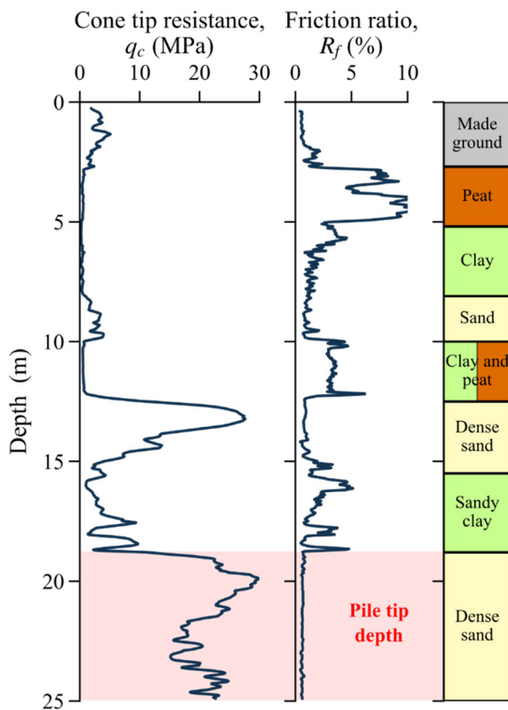
Fig. 5. Typical CPT profile in Amsterdam, near the GIKEN demonstration case
