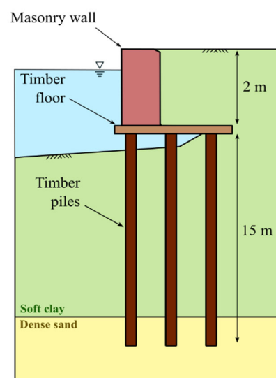
Fig. 2 An example of an urban quay wall built before the 20 th century
