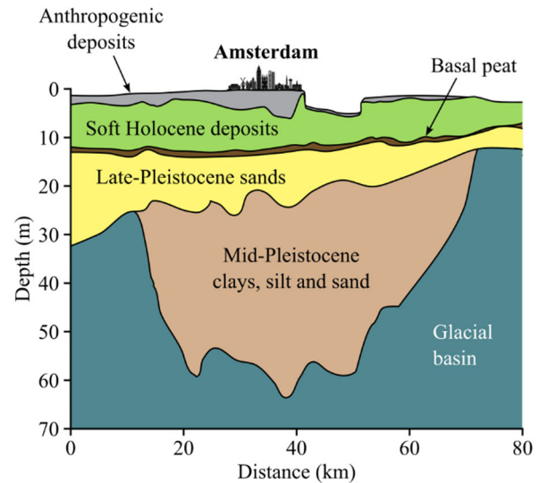
Fig. 3. Geological cross-section of Amsterdam
